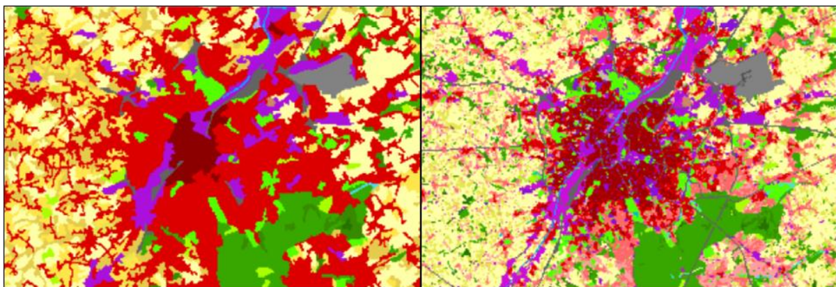
Figure 4: Differences between the original CLC 2012 (left) and the CLC after spatial and thematic refinement (right) for the area surrounding Brussels, Belgium.
